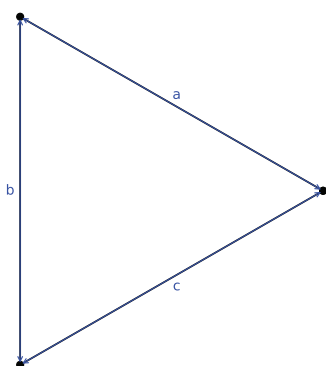
3-sided Polygon
