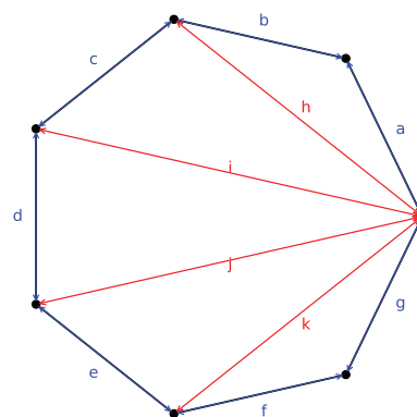
7-sided Polygon
