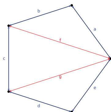
5-sided Polygon
