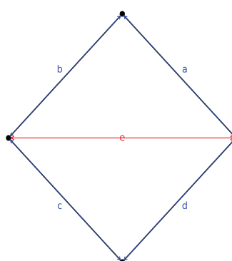
4-sided Polygon
